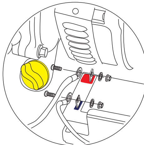
Figure 15 - Battery Connections
