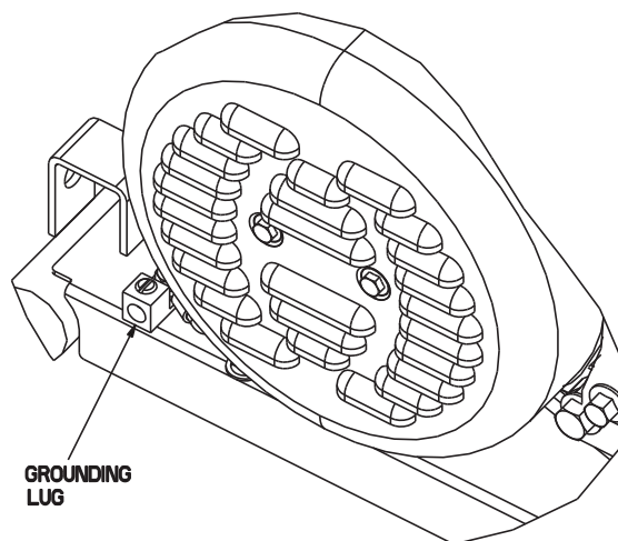
Figure 8 - Grounding the Generator
