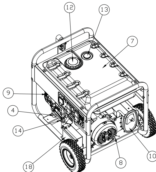
Figure 4 - Generator Controls
